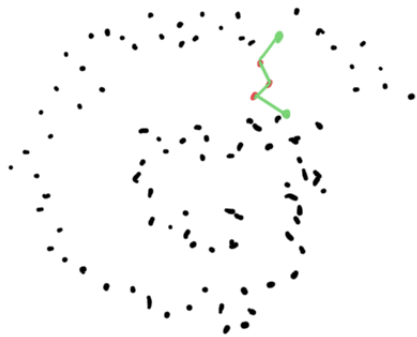
Figure 30: With extra noisy points (red), the geodesic distance can get corrupted.
