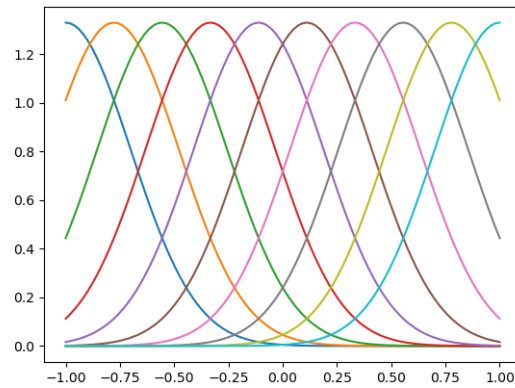
Figure 32: Gaussian basis functions over the interval [-1, 1] with standard deviation of 0.3
