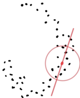
Figure 31: Local linear embedding assumes that the data is locally linear.
