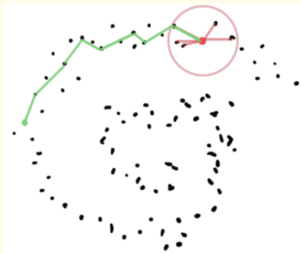
Figure 29: The classical example is the spiral manifold. The data lies in this manifold, and the geodesic distance helps us gain an accurate distance metric within this data.
