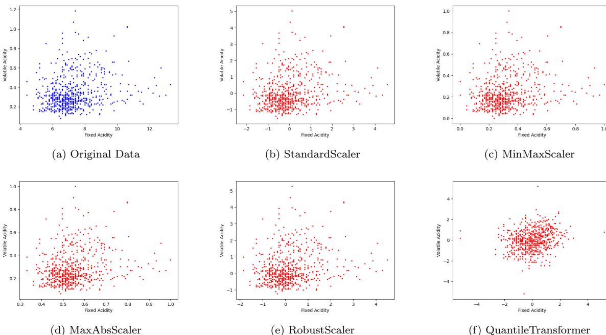
Figure 34: The StandardScaler simply standardizes the data to have 0 mean and unit variance.
