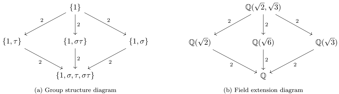
Figure 19: Lattice diagrams showing group structure and corresponding field extensions
