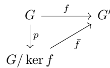
Figure 6: Given f and the projection map p : G \rightarrow G/\ker f , this induces an isomorphism \bar{f} such that f = \bar{f} \circ p .
