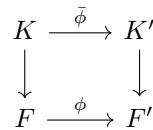
Figure 18: Commutative diagram.
